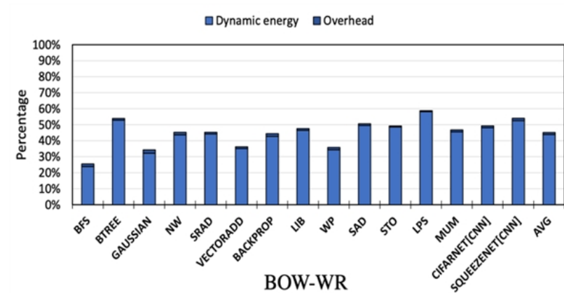
Fig 1: shows the dynamic energy normalized to the baseline GPU for BOW-WR across fifteen different benchmarks. The small segments on top of each bar represent the overheads of the structures added by the idea. Dynamic energy savings in Fig 1 are due to the reduced number of accesses to the register file as BOW-WR shields the RF from unnecessary read and write operations.
