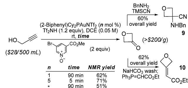
Scheme 2. A One-Step Synthesis of Oxetan-3-Ones and Its Synthetic Conversion without Purification
